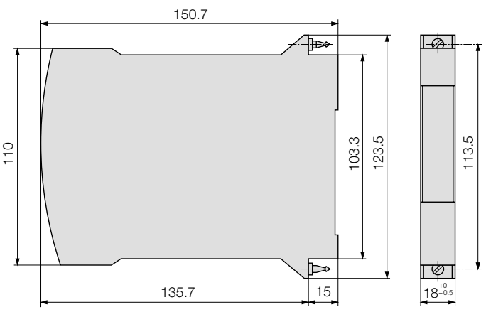
Fig. 3. SIRAX TV 808 in housing B17.
