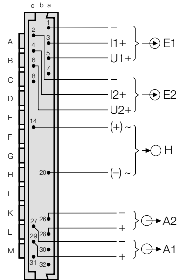
SIRAX TV 808 Rear
